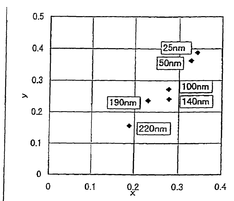
Bytron FILM THICKNESS vs. LIGHT-EMITTING CHROMATICITY
